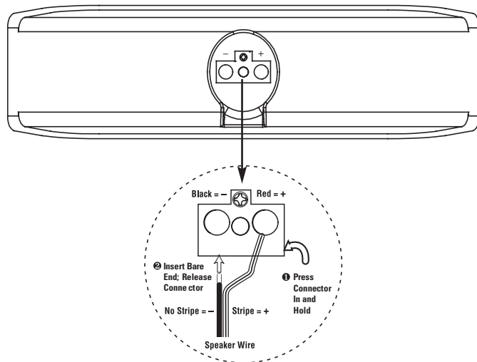
Figure 5. Wiring diagram shows polarity connections for a center channel.
